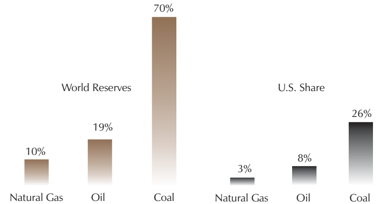
Percentage of Fossil Fuel Energy Reserves (coal unit equivalents)
